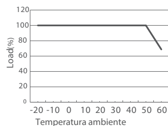
Curva Derating
