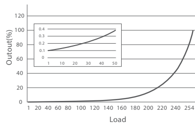
Curva Dimming
